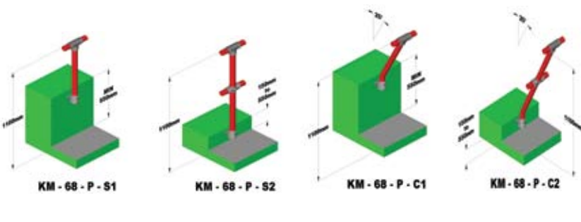
Kee Modules® side fix mounted, handrail tube in-line
