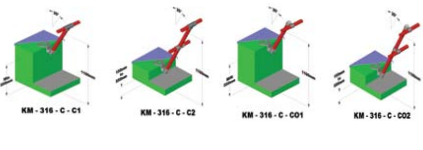
Kee Modules® for mounting under aluminium coping, handrail off-set or in-line
