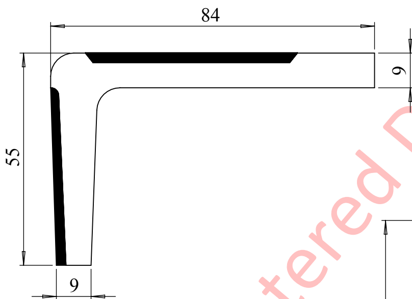
Side view scale 1:1
