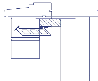
Sill detail
