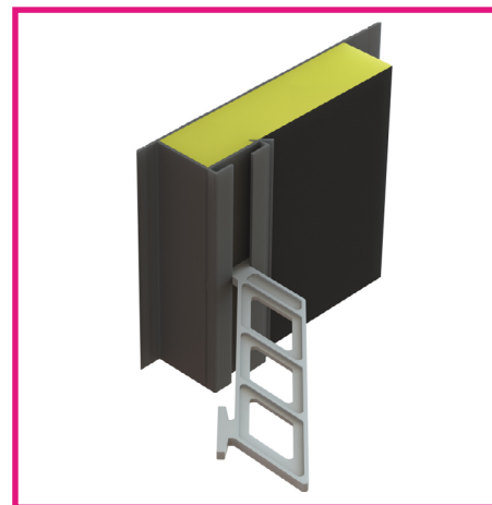
Thermo-loc FR30 Single Profile
