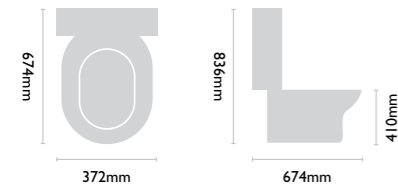
Navlin Standard-Height Close-Coupled Toilet Pan | 23571
