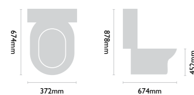
Navlin Cistern with Raised Push Button Flush | 23574
