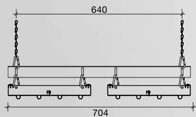
Spacing of suspension points per bar
