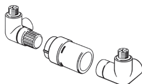
RTX sensor, RA-URX left mounted and RLV-X right mounted.
