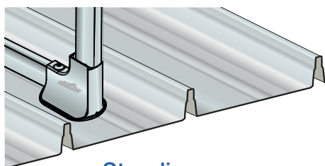
Standing seam with bracket
