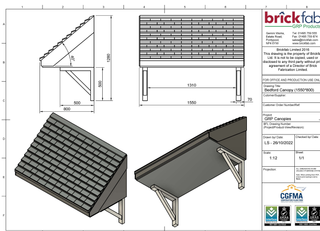
Canopy Dimensions (mm)
