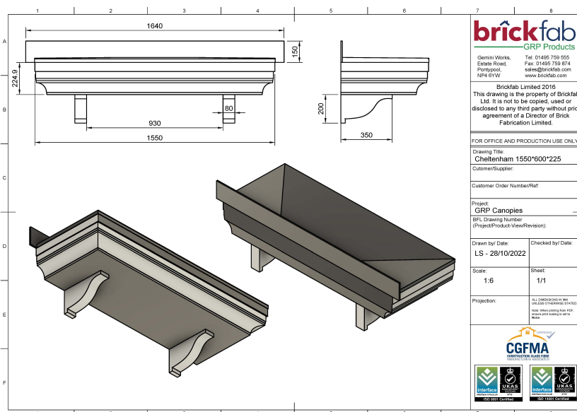
Canopy Dimensions (mm)
