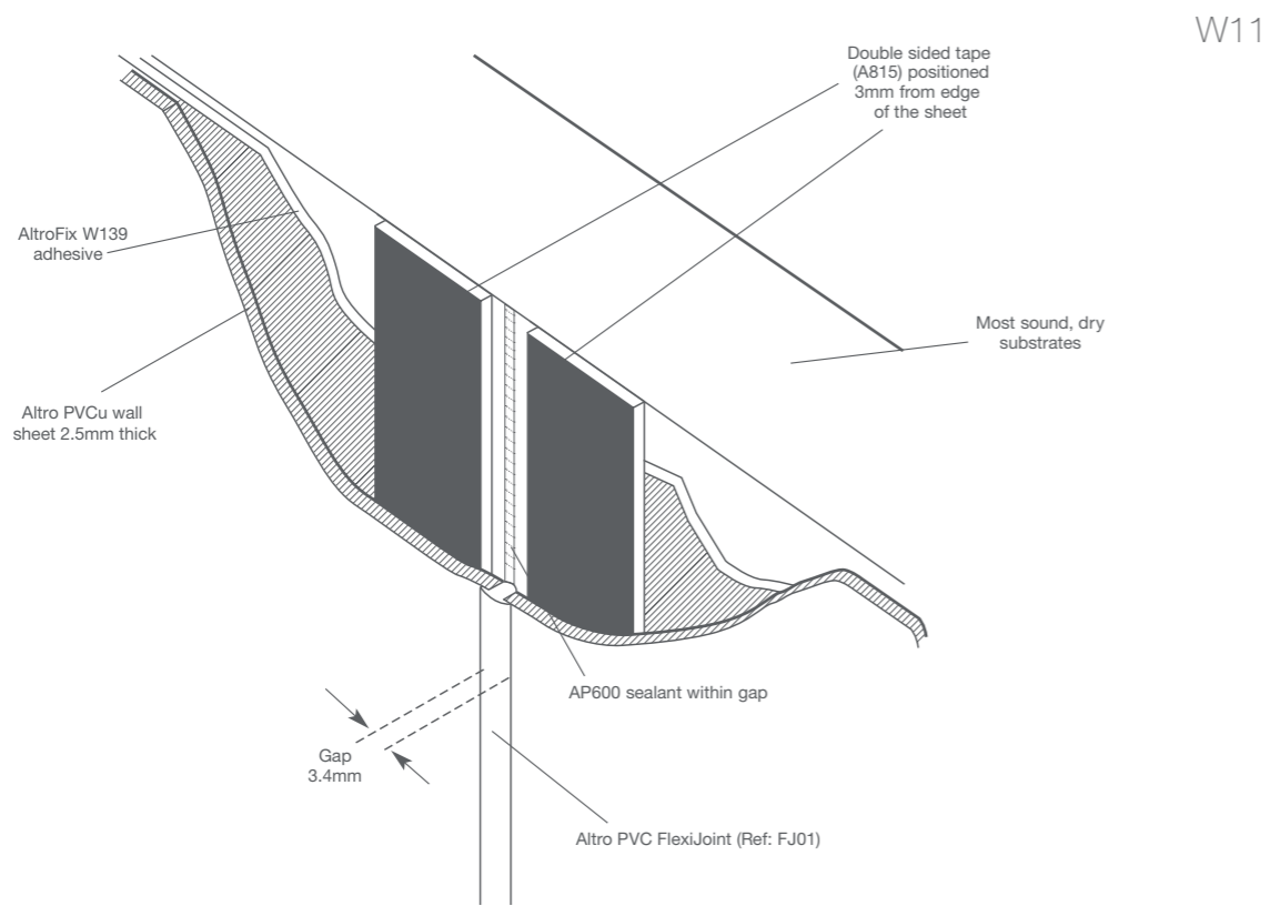
Altro wall sheet to Altro Whiterock FlexiJoint detail
