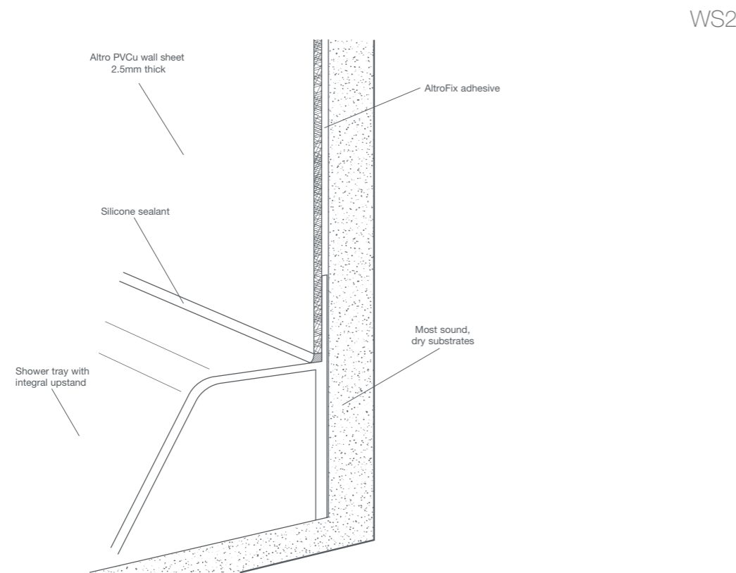
Altro Whiterock hygienic PVCu wall system to shower tray with integral upstand detail
