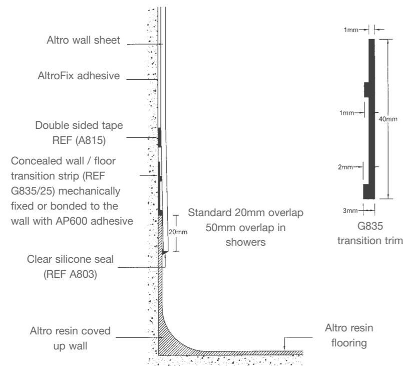
Concealed transition strip
