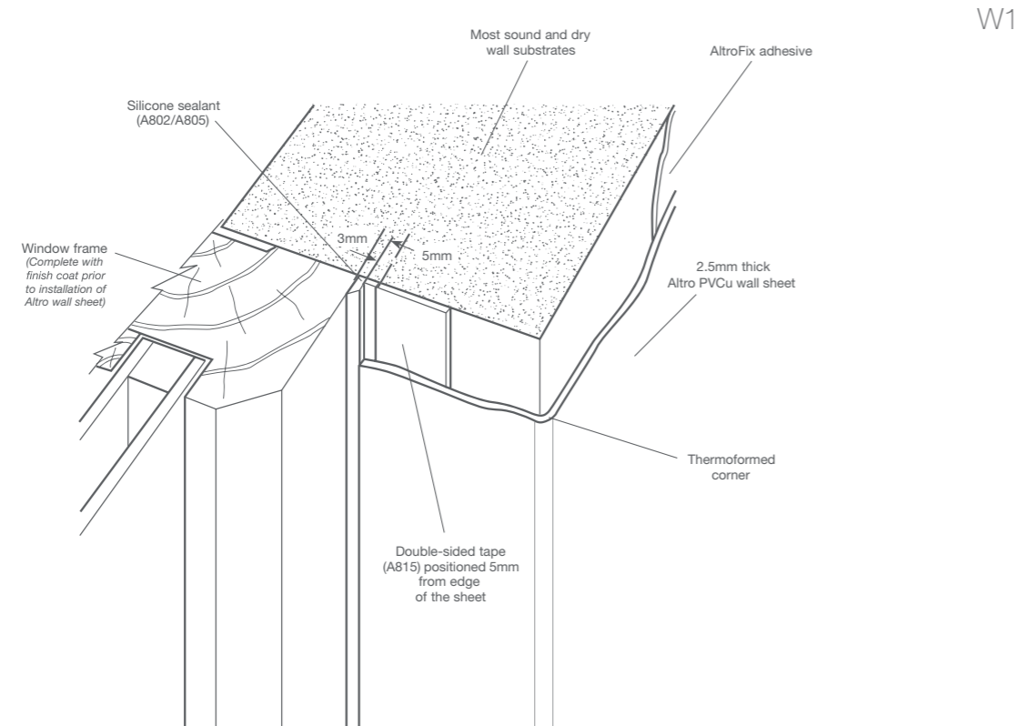
Altro wall system to window / door frame detail
