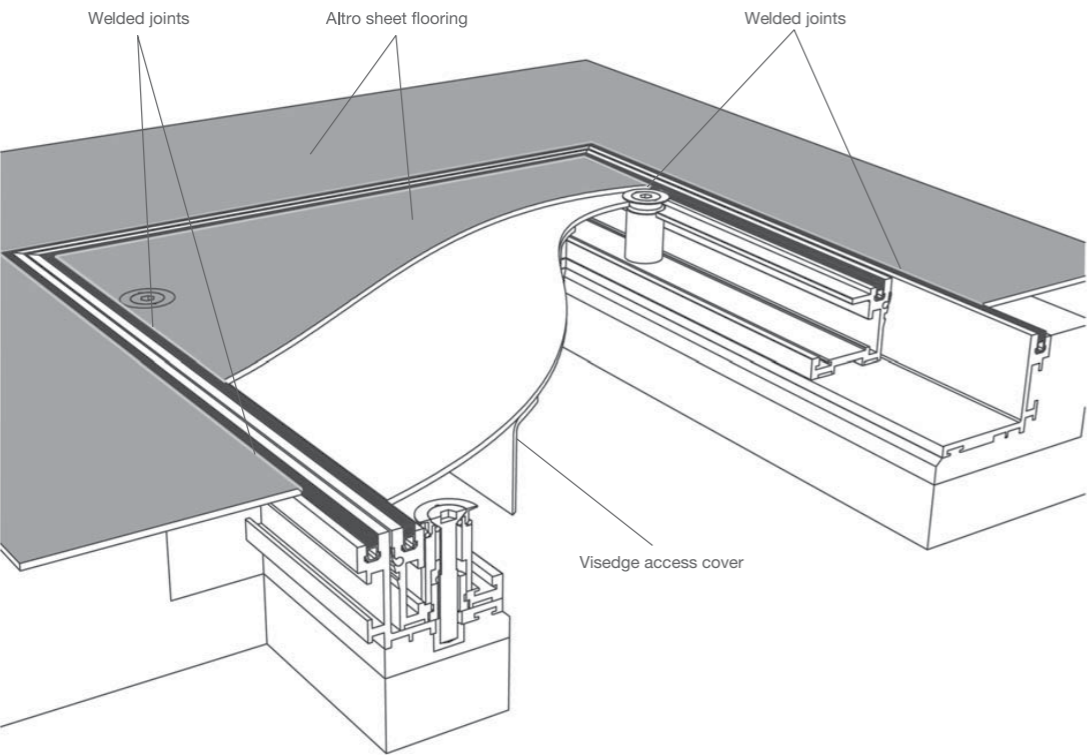
Transition with access covers
