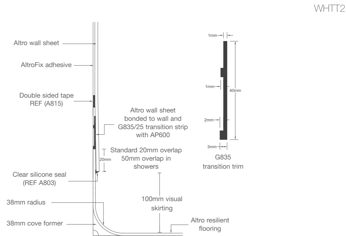
Concealed transition strip
